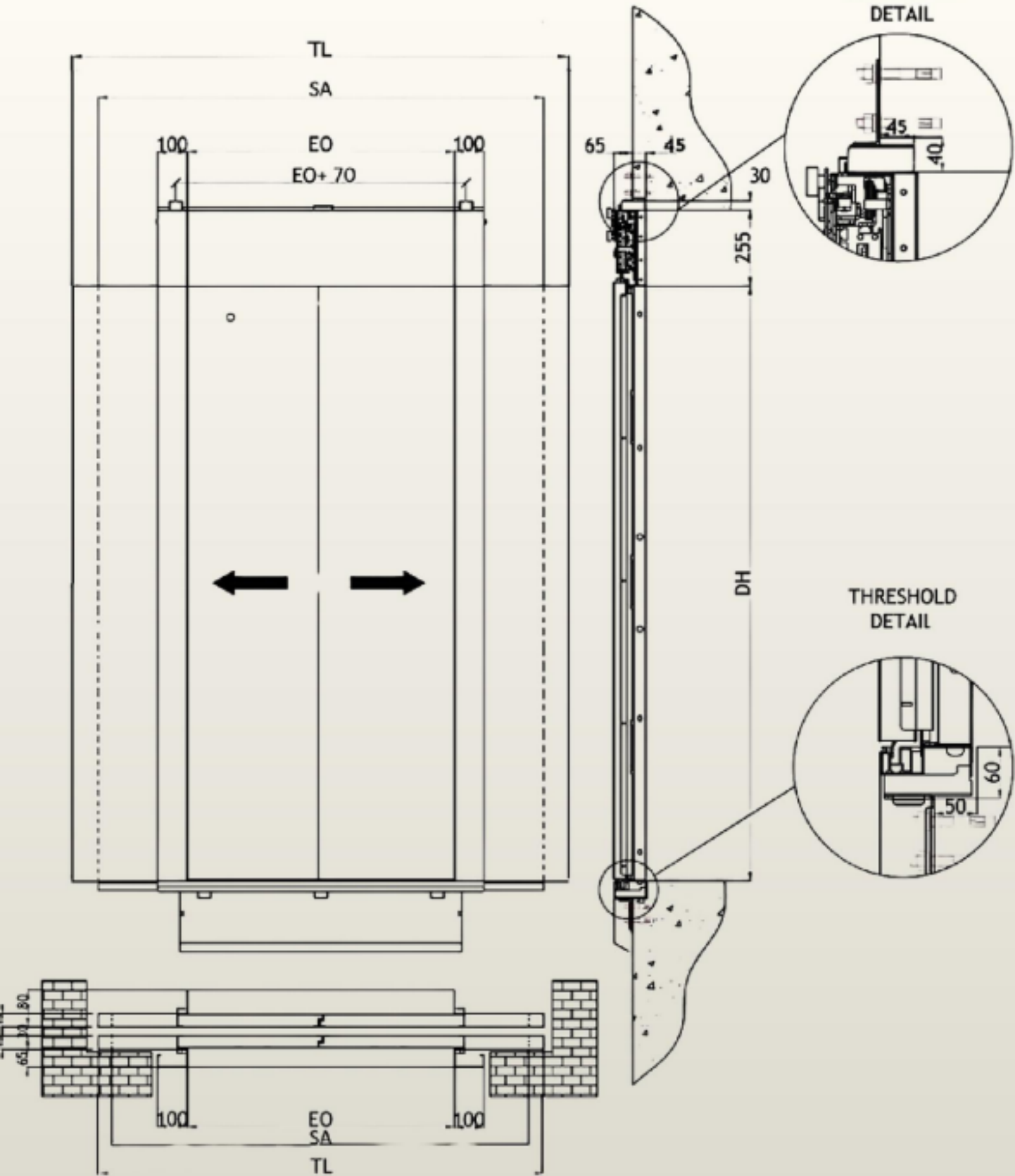
Technical Dimensions
